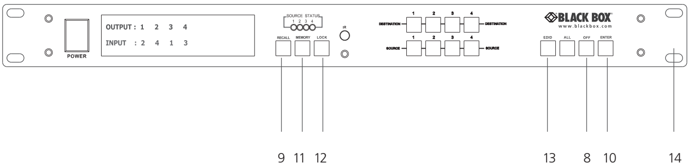
Figure 2-2. Front-panel diagram #2.
